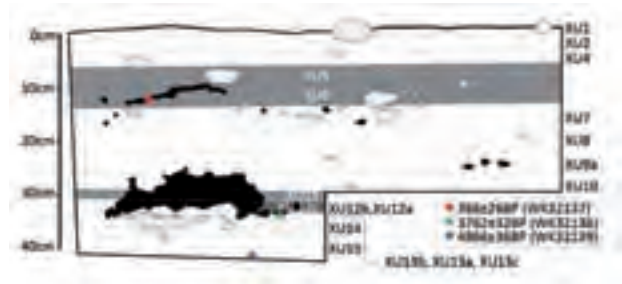
Figure 3 East section of the Weld-RS-0731 excavation. Key: charcoal = black; rocks = light grey; excavation units from which charcoal was sampled for this study are shaded in dark grey. Uncalibrated radiocarbon date sample locations are labelled.
